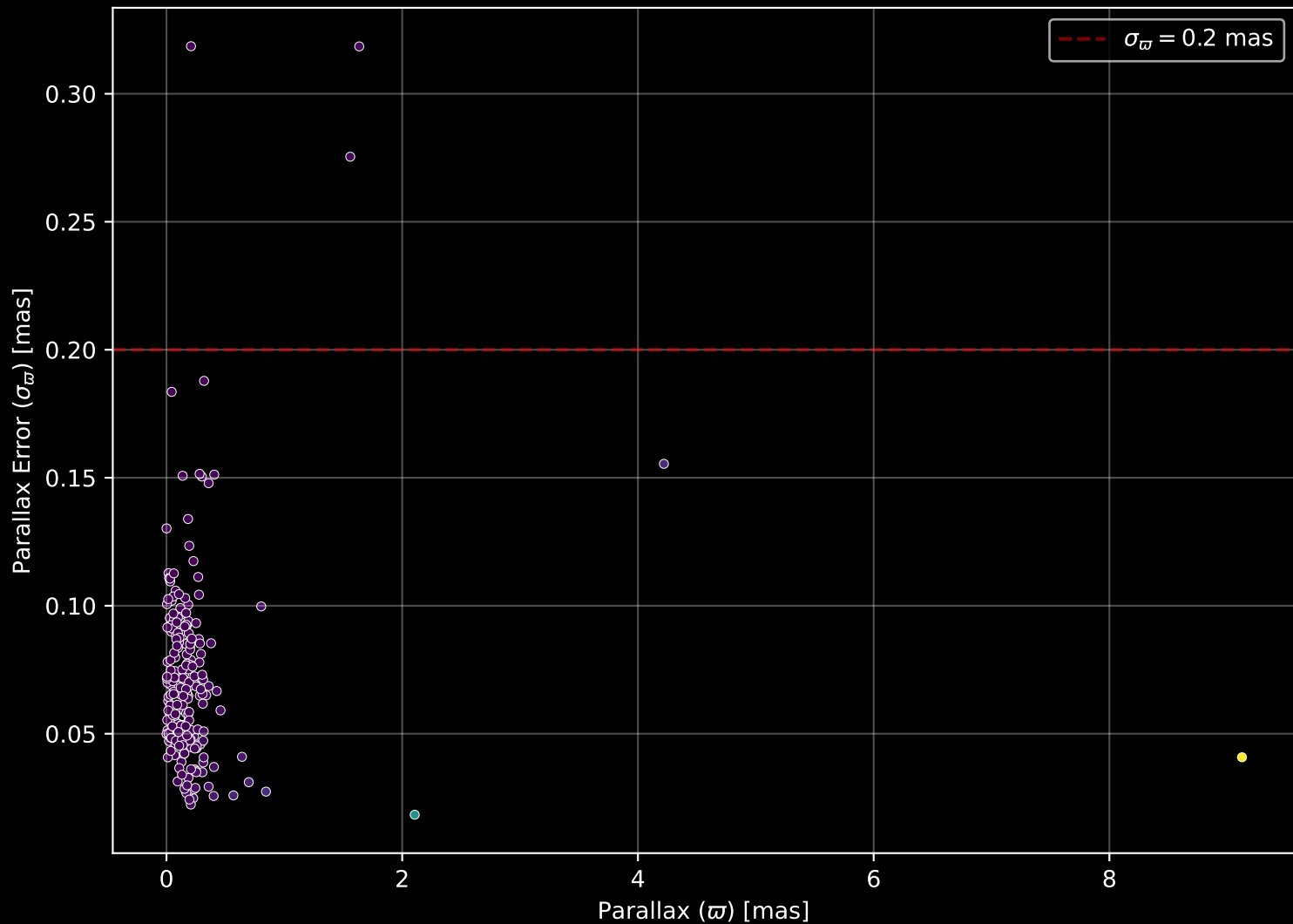
APOGEE DR17 Field: [005+02] Parallax Quality (n= 219)
