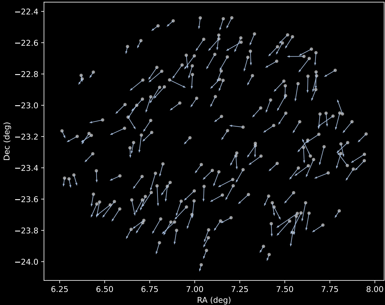
APOGEE DR17 Cluster 1 Proper Motion Vectors (n=176)
