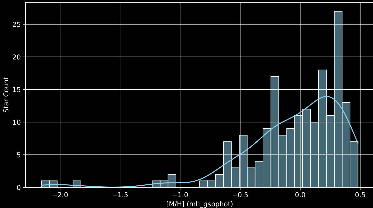
APOGEE DR17 Field: [005+02 [M/H] (mh_gspphot) (n= 188)
