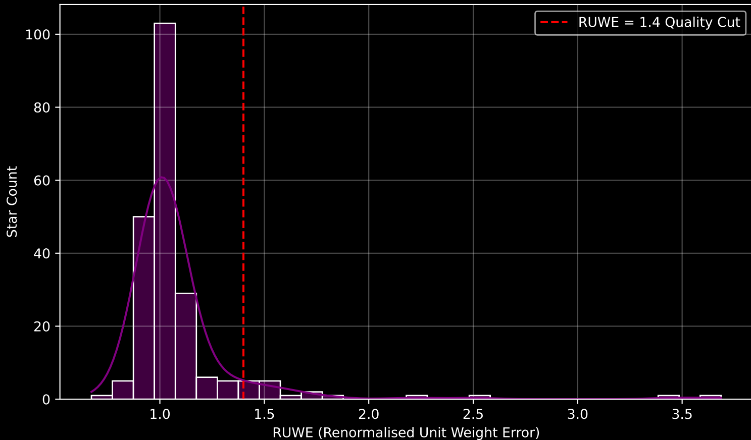
GAPOGEE DR17 Field [005+02] RUWE Distribution (n= 217)
