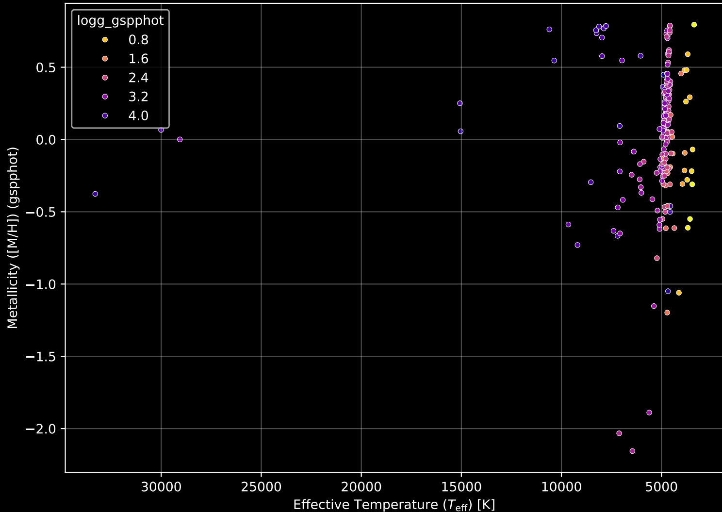
APOGEE DR17 Field: [005+02] Stellar Population Parameters (n= 219)
