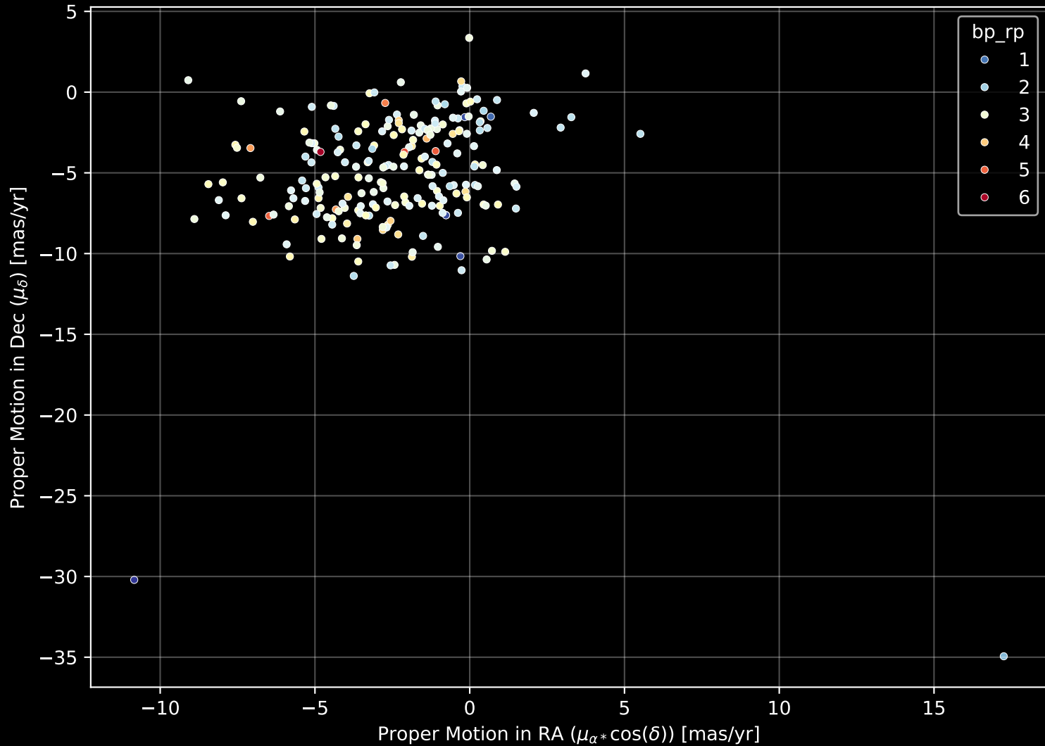
APOGEE DR17 Field: [005+02] Proper Motion Diagram (n= 219)
