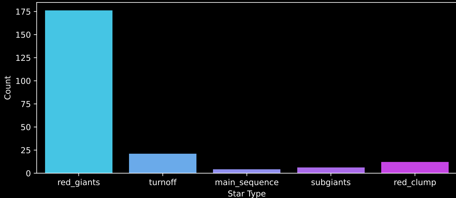
APOGEE DR17 Field: [005+02] Count plot of Star Type
